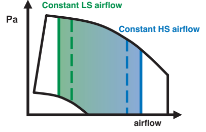
SILVERTOP® + QUATTRO® Operation PROPORTIONAL ventilation between two CONSTANT airflows per fan. Except for SILVERTOP® 06 and 08.
