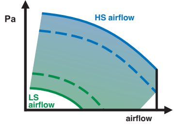
SILVERTOP® + DIVA® Operating PROPORTIONAL ventilation between two airflows (LS/HS) per fan.
