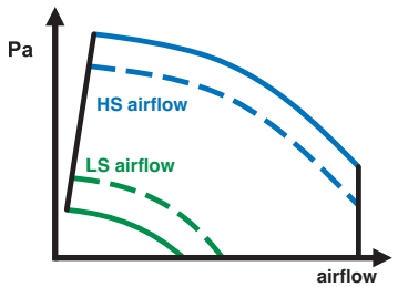
SILVERTOP® ECO Operating Selection of 1 or 2 different airflows (LS/HS) per fan. Except for SEASON, 1 airflow adjustable with potentiometer
