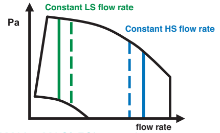
CARMA® + MAC2 EC® operation Optional 1 or 2 CONSTANT flow rates by fan (except CARMA® 9008)
