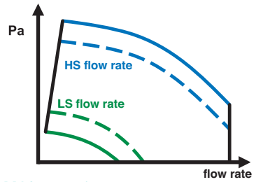
CARMA® operation 1 or 2 flow rates as required (Low Speed(LS)/High speed(HS)) per fan Except SEASON, 1 flow adjustable spleen by potentiometer
